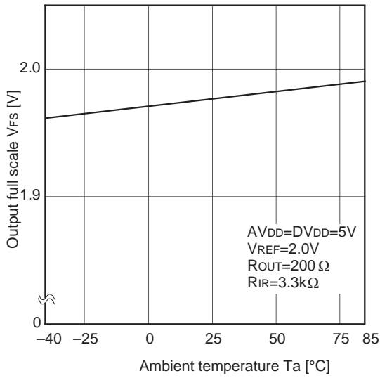
Output full scale voltage vs. Ambient temperature
